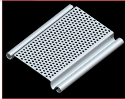
3mm Round hole @ 5mm pitch, Staggered, Flat profile
